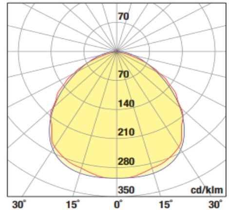
SMD UNIVERSAL 12-24Vdc - 110°
